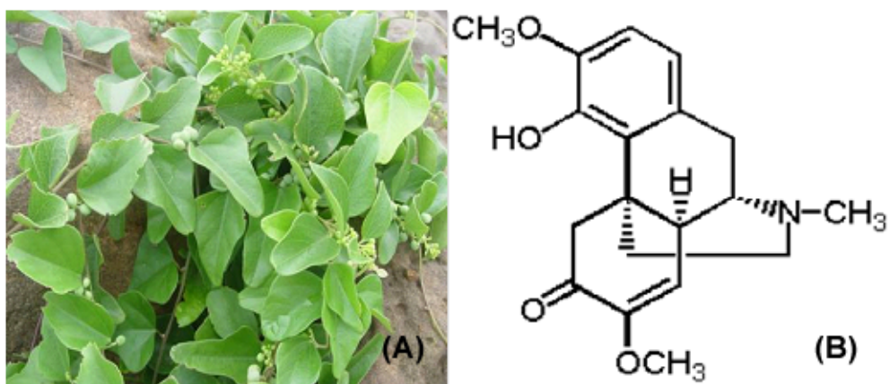
Fig. 1S Photograph of Caulis sinomenii (A) and the chemical structure of sinomenine (B).
