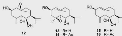
► Fig. 3 Chemical structures of compounds 12–16.
