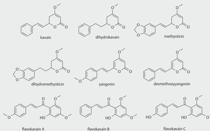
► Fig. 1 Chemical structure of kavalactones and flavokavains analyzed in this study.
