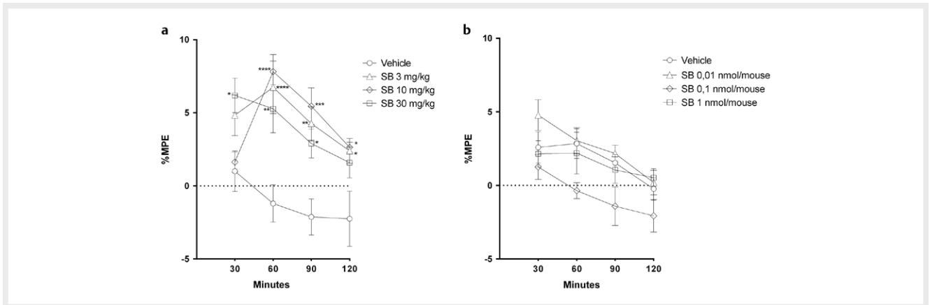
► Fig. 2 Time course of the effects of systemic (3, 10, 30 mg/kg) and intrathecal (0.01, 0.1, 1 nmol/mouse) administrations of the 5-HT 6 receptor antagonist SB-258585 on thermal hyperalgesia in diabetic mice on day 15 after streptozocin injection (2-way analysis of variance followed by Bonferroni t test, *P<0.05, **P<0.01, ***P<0.001, ****P<0.0001, vs. control group).
