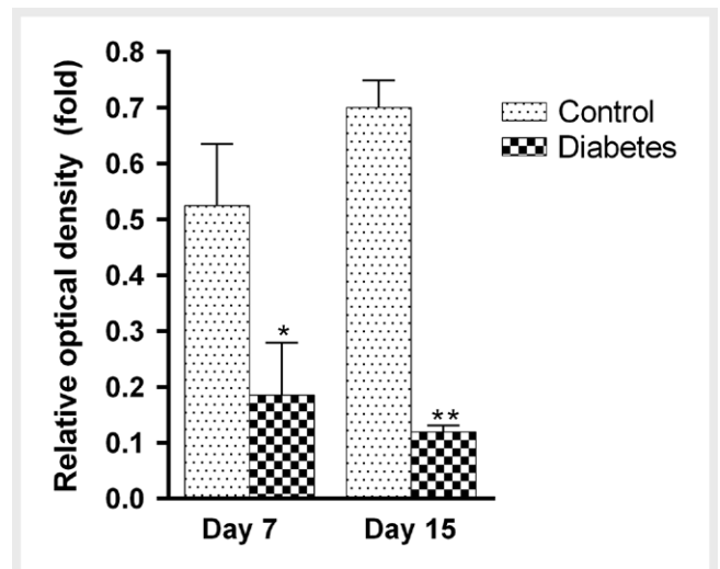
► Fig. 4 Western blot analysis of lumbar dorsal spinal cord for 5-HT 6 expression in control and diabetic mice on days 7 and 15 after respective vehicle or streptozocin injections (unpaired t-test, *P<0.05, **P<0.0001 vs. control group).
