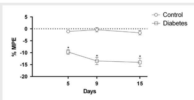
► Fig. 1 Thermal hyperalgesia induced by diabetes. Thermal thresholds for the hot plate tests were determined on days 5, 9 and 15 after streptozocin injection (150 mg/kg, i.p.; 2-way analysis of variance followed by Bonferroni t test, * P<0.0001, vs. control group).
