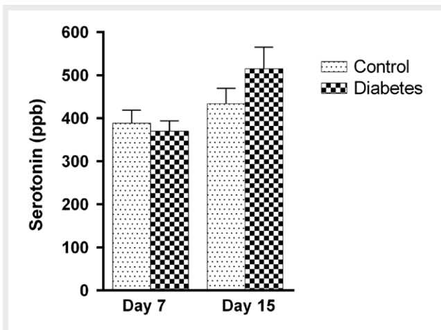
► Fig. 3 LC/MS/MS analysis of lumbar dorsal spinal cord for serotonin content in control and diabetic mice on days 7 and 15 after respective vehicle or streptozocin injections. No significant change was observed (unpaired t-test).
