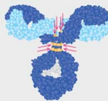
Natural cysteine residues 8 Conjugation sites DAR 3–8 (brentuximab-vedotin, T-DXd)
