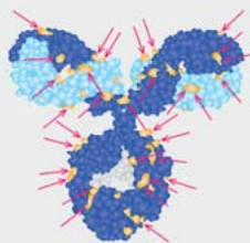
Natural lysine residues >70 Conjugation sites DAR 3–4 (T-DM1)
