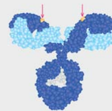
Engineered cysteine residues 2 Conjugation sites DAR 1–2
