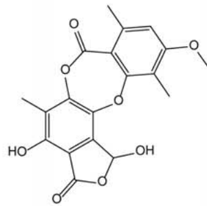
Hypostictic acid
