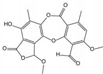
8'-O-methylstictic acid
