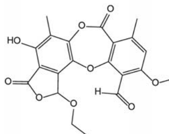
8'-O-ethylstictic
