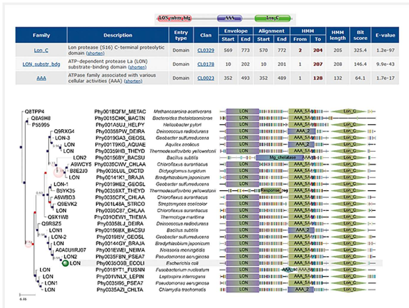
► Fig. 2 Results of domain and phylum analysis of the Lon protease using PhylomeDB [21]. Lon is conserved among major lineages of the domain bacteria.
