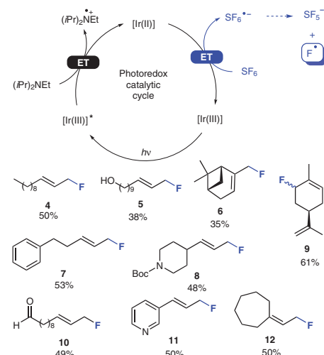
Scheme 3 Photoredox catalytic activation of \text{SF}_6 by \text{Ir}(\text{ppy})_2(\text{dtbbpy})\text{PF}_6 for the deoxyfluorination of allylic alcohols, e.g., 1 to allylic fluorides 2 and 3 (top), the proposed photoredox catalytic cycle (middle) and examples of the product scope 4–12 (bottom)
