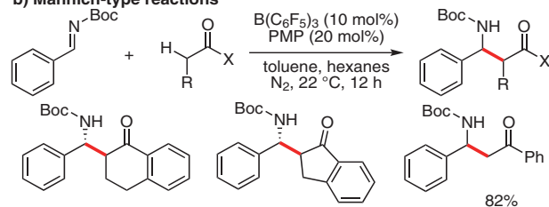
Figure 5 Frustrated Lewis pair catalysed C–C bond formation by a) cycloisomerizations b) Mannich-type reactions c) rearrangements d) Diels–Alder reactions and e) C–C couplings
