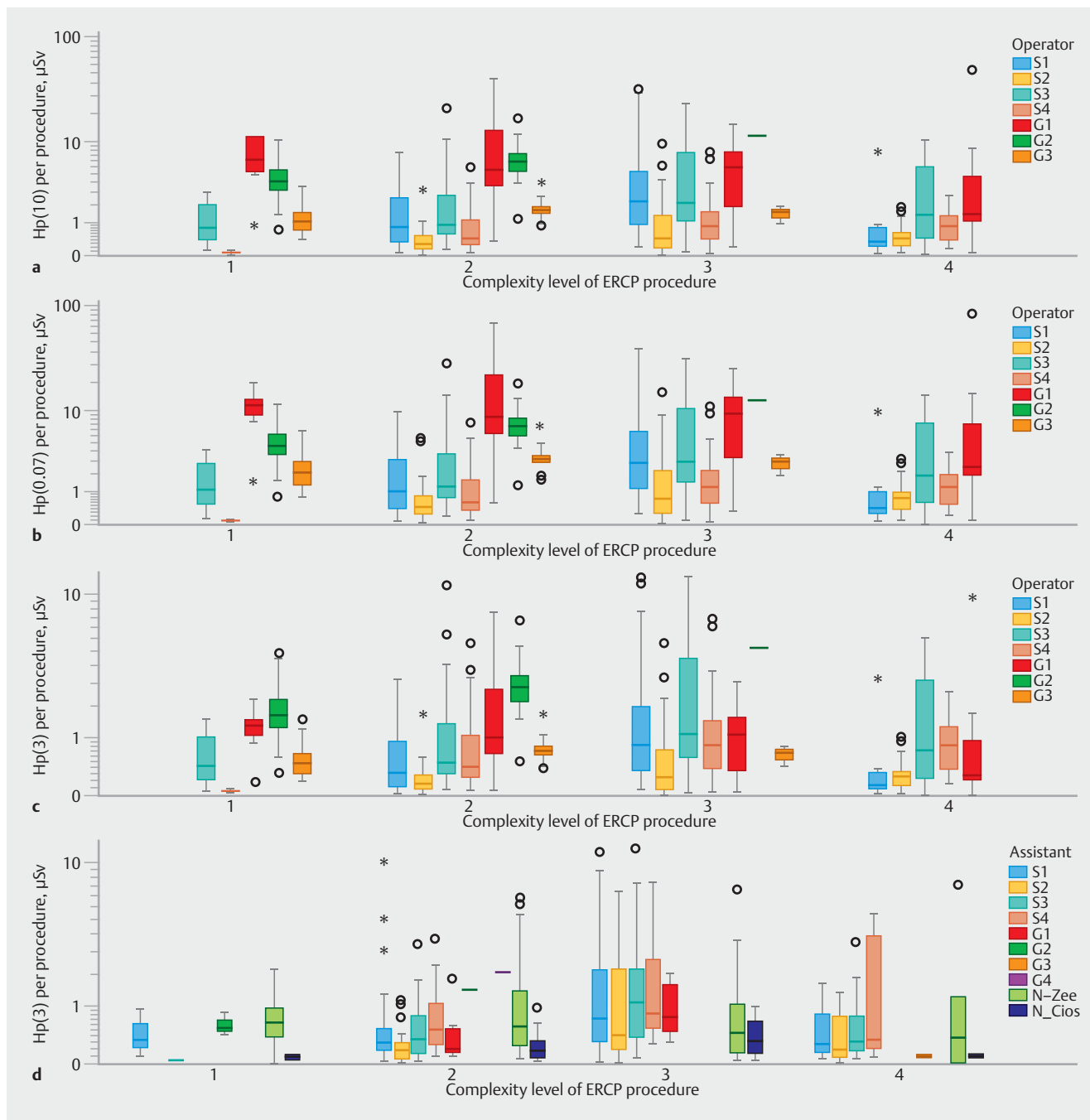
► Fig. 1 Occupational radiation doses in a single ERCP intervention according to complexity level of procedure. Operator-specific personal dose equivalents a H_p(10) , b H_p(0.07) , and c H_p(3) and d assistant-specific eye lens dose equivalent H_p(3) per ERCP procedure. The H_p(10) and H_p(0.07) shown represent doses estimated from TLD-100 measurements. Logarithmic scale is used on the y-axis.
