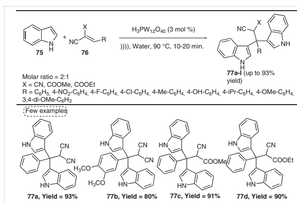
Scheme 26 Synthesis of various bis(indole) derivatives
