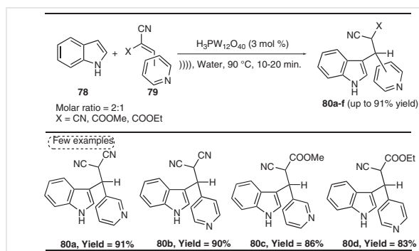
Scheme 27 Synthesis of mono-indolyl derivatives
