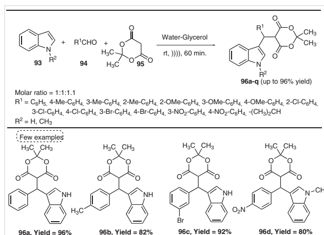
Scheme 31 Synthesis of 3-substituted indoles
