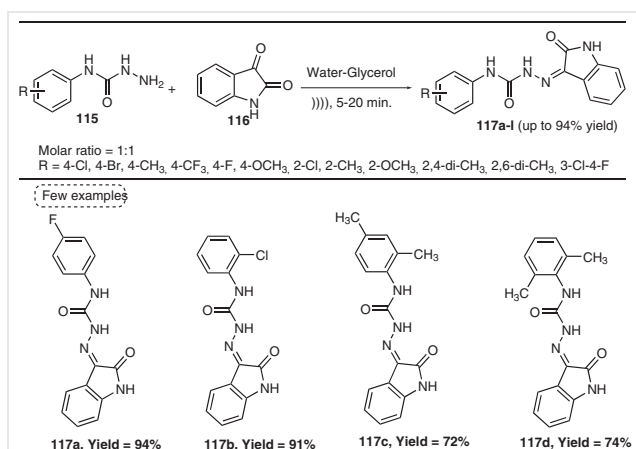
Scheme 40 Synthesis of N-(substituted phenyl)hydrazine carboxamide derivatives
