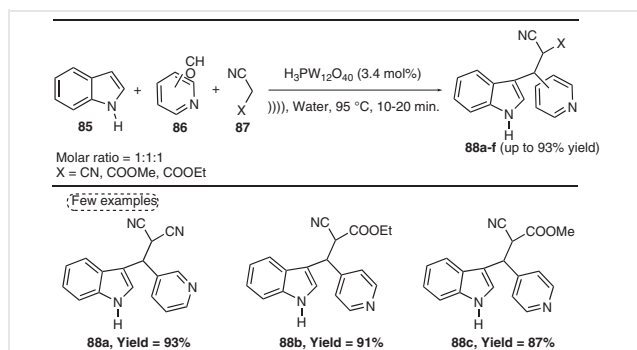
Scheme 29 Synthesis of mono-indolyl derivatives
