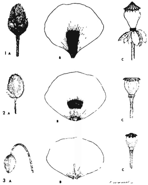
Fig. 2. Taxonomic characters of Papaver bracteatum [1], P. pseudo-orientale [2] and P. orientale [3]. (A = bud; B = petals; C = mature capsules). After GOLDBLATT [13].
