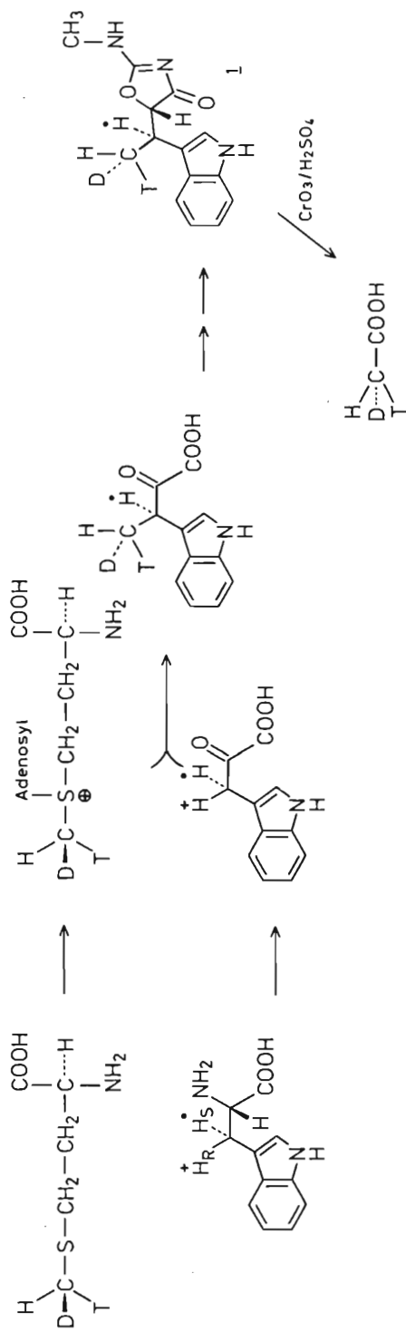
Fig. 6. Summary of the stereochemical course of the C-methylation reaction involved in indolmycin biosynthesis.
