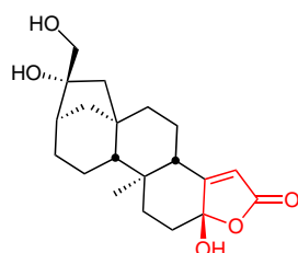
Tricalysiolide B
