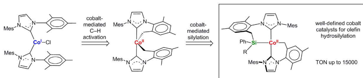
Figure 1 Synthetic approach for the silyl donor functionalized N-heterocyclic carbene–cobalt catalyst
