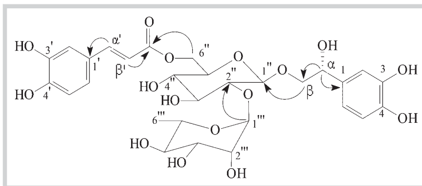
Fig. 1 Key HMBC correlations (H → C) of 1.
