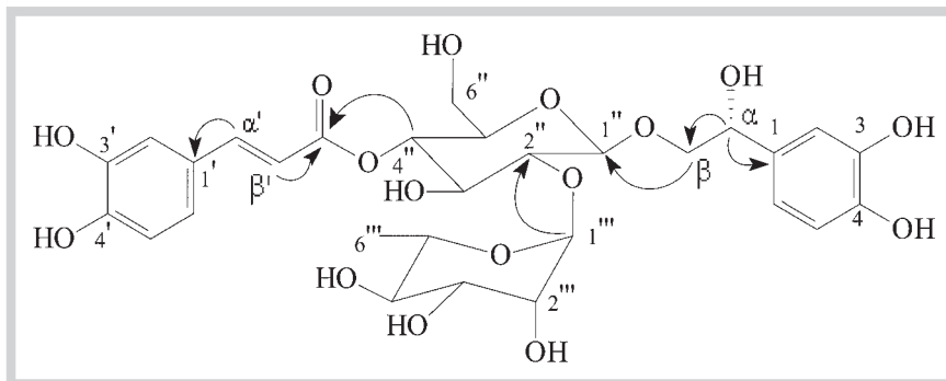
Fig. 2 Key HMBC correlations (H → C) of 2.
