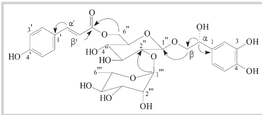
Fig. 4 Key HMBC correlations (H → C) of 4 .
