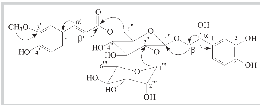
Fig. 5 Key HMBC correlations (H → C) of 5 .
