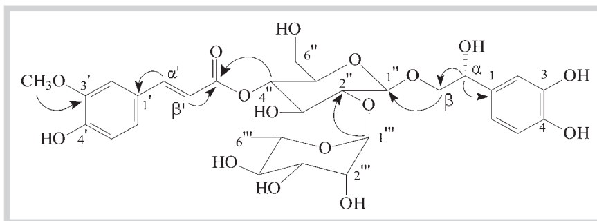
Fig. 3 Key HMBC correlations (H → C) of 3.
