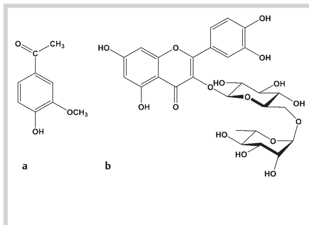
Fig. 1 Chemical structure of apocynin (a) and rutin (b).
