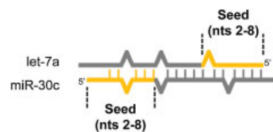
Fig. 3 MicroRNA-microRNA binding. Mature microRNAs can bind in a sequence-specific manner to each other, as demonstrated by cross-linking, ligation and sequencing of hybrids (CLASH). Illustrated here is the antiparallel microRNA duplex containing let-7a and miR-30c, adapted from Helwak et al. 22 The 5' terminus and seed region of each microRNA are indicated in yellow (nucleotides 1–8) and the remaining microRNA is in grey. Vertical “ladder rungs” indicate Watson-Crick base pairing, whereas the absence of a rung indicates a mismatch (i.e., within the miR-30c seed). Single nucleotide bulges (either symmetric or asymmetric) are depicted as a triangular deviation of the backbone.
