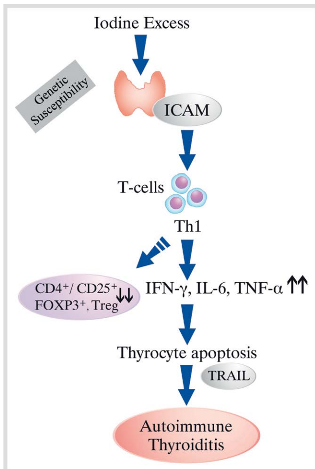
Fig. 1 High iodine intake may in susceptible individuals lead to an increased expression of ICAM-1 on thyroidal follicle cells, induce T helper cells to differentiate towards T helper 1 (Th1), decrease CD4+/CD25, FOXP3 and TREG, increase cytokine secretion, induce apoptosis via abnormal TRAIL expression and mediate thyroid destruction. ICAM: Intracellular adhesion molecule; TRAIL: Tumor necrosis factor (TNF) related apoptosis-inducing ligand (TRAIL); FOXP3: Forkhead/winged helix transcription factor p3 (FOXP3). (Color figure available online only).
