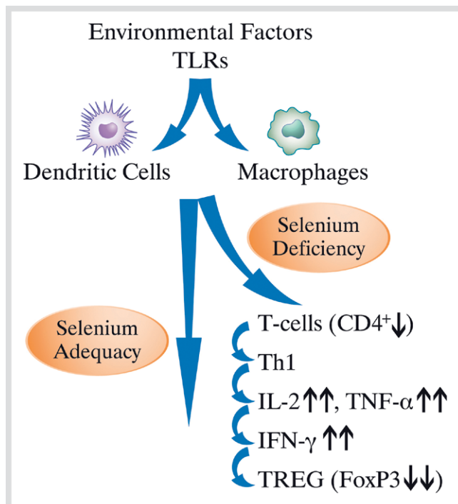
Fig. 2 Increased Se intake induces, via activation of the T cell receptor (TCR), differentiation of CD4+T cells into CD25+Foxp3+T regulatory cells (TREG). Adequate levels of Se intake do not affect T cells and T helper cells (Th0) vs. Th1 or Th2 differentiation. In contrast, Se deficiency, as an environmental factor, increases T-cell activation, while the T helper-1 (Th1)/T helper-2 (Th2) ratio may shift to a Th1-type response, increasing such cytokines as IL-2, TNF- \alpha , IFN- \gamma , thereby reducing CD25+T regulatory cells (TREG)+Foxp3 and in parallel inhibiting an activation of dendritic cells and macrophages by Toll-like receptor (TLR) cells [57, 61]. TREG likely responds to different ligands for TLRs, thus the TLRs may exert different effects on TREG, depending on the degree of inflammation, resulting in more suppression or, in contrast, abrogation of suppression [68]. (Color figure available online only).
