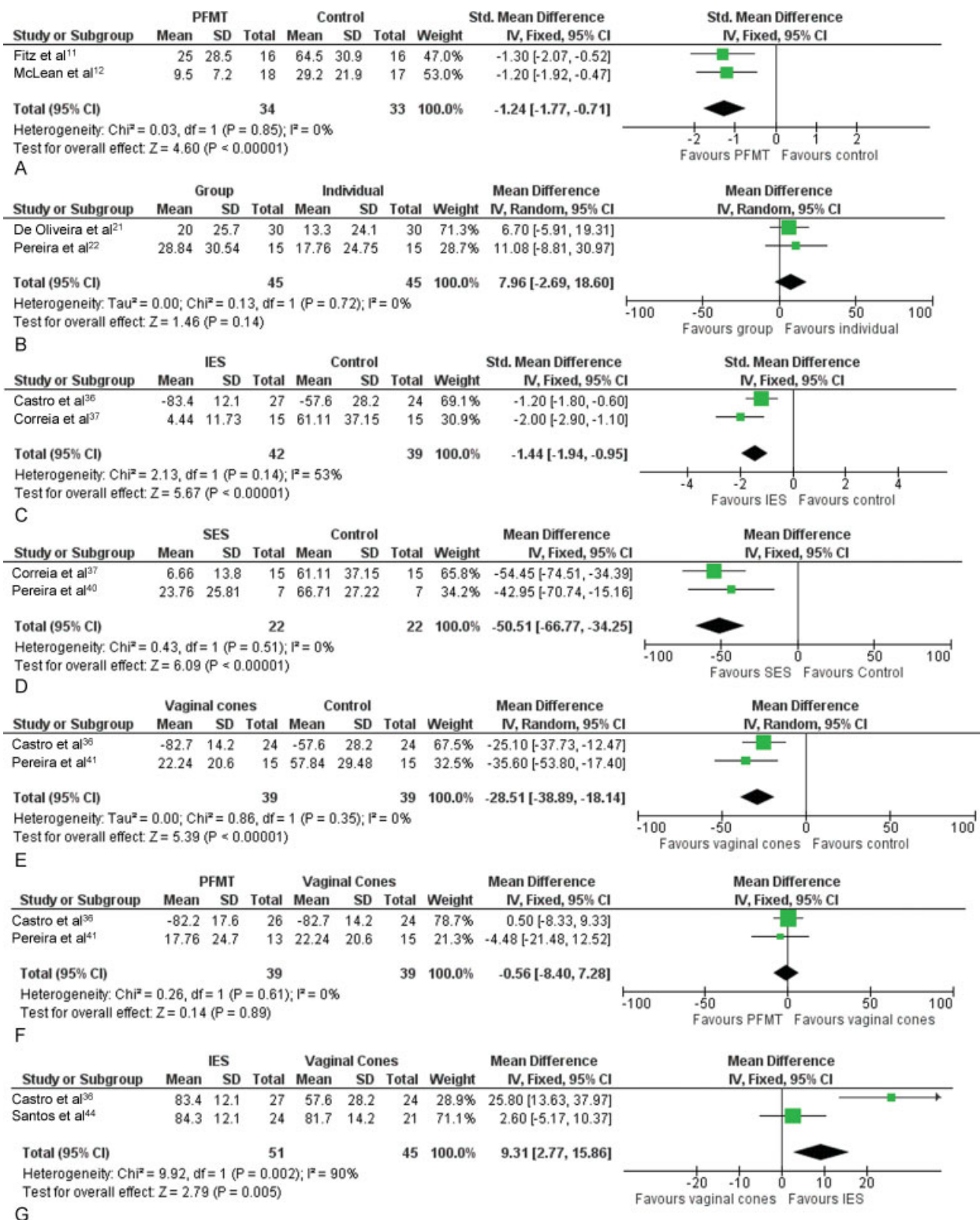
Fig. 2 Meta-analyses for the outcome "Incontinence-specific quality of life." (A) PFMT vs control; (B) Group PFMT vs individual PFMT; (C) Intravaginal electrical stimulation vs control; (D) Superficial electrical stimulation vs control; (E) Vaginal cones vs control; (F) PFMT vs vaginal cones; (G) Intravaginal electrical stimulation vs vaginal cones. Abbreviations: SD, standard deviation; IV, inverse variance; IES, intravaginal electrical stimulation; SES, superficial electrical stimulation.
