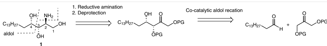
Scheme 1 Retrosynthesis of D -lyxo-[2 S ,3 S ,4 S ]-phytosphingosine ( 1 ); PG = protective group
