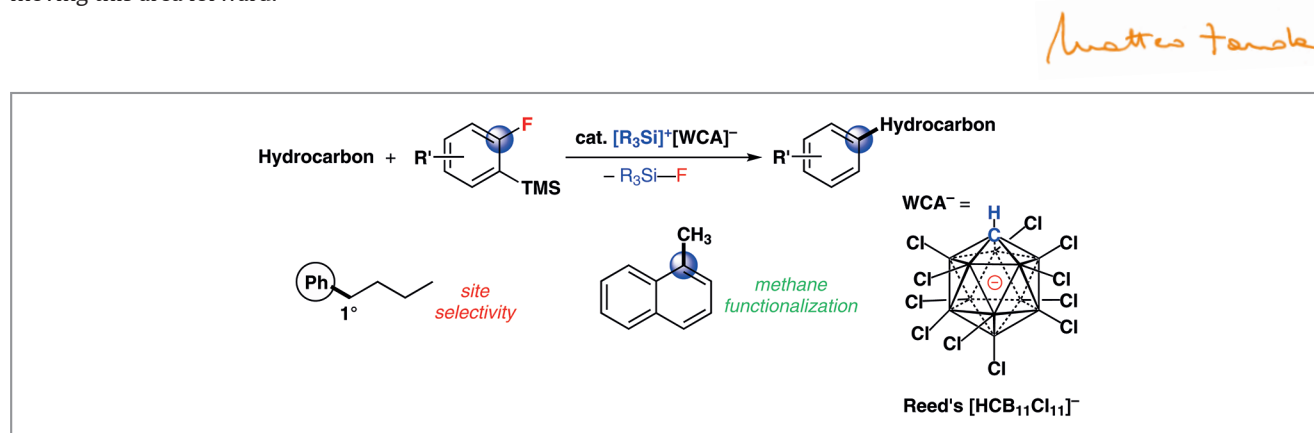
Figure 1 The novel synthetic methodology
