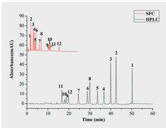
► Fig. 4 Separation of the 12 flavonoids in both SFC and HPLC modes. Peak assignment: 1. Kaempferide, 2. Baicalein, 3. Kaempferol, 4. Luteolin, 5. Quercetin, 6. Morin, 7. Myricetin, 8. Baicalin, 9. Hyperoside, 10. Luteoloside, 11. Myricitrin, 12. Buddleoside. Reproduced with permission from [51] [rerif].
