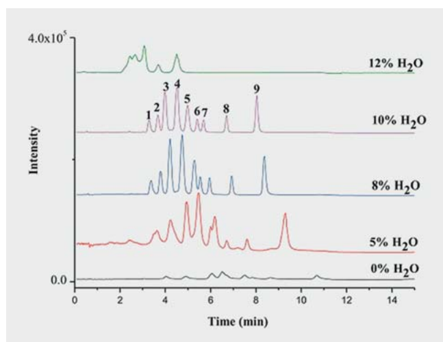
► Fig. 3 Effect of water content in the mobile phase on the separation of nine kudinosides from Ilex latifolia leaves. Peak assignment: 1. Kudinoside F, 2. Kudinoside A, 3. Ileukudinoside G, 4. Kudinoside E, 5. Kudinoside C, 6. Kudinoside G, 7. Latifolioside Q, 8. Latifolioside H, 9. Kudinoside O. Reproduced with permission from [42] [rerif].
