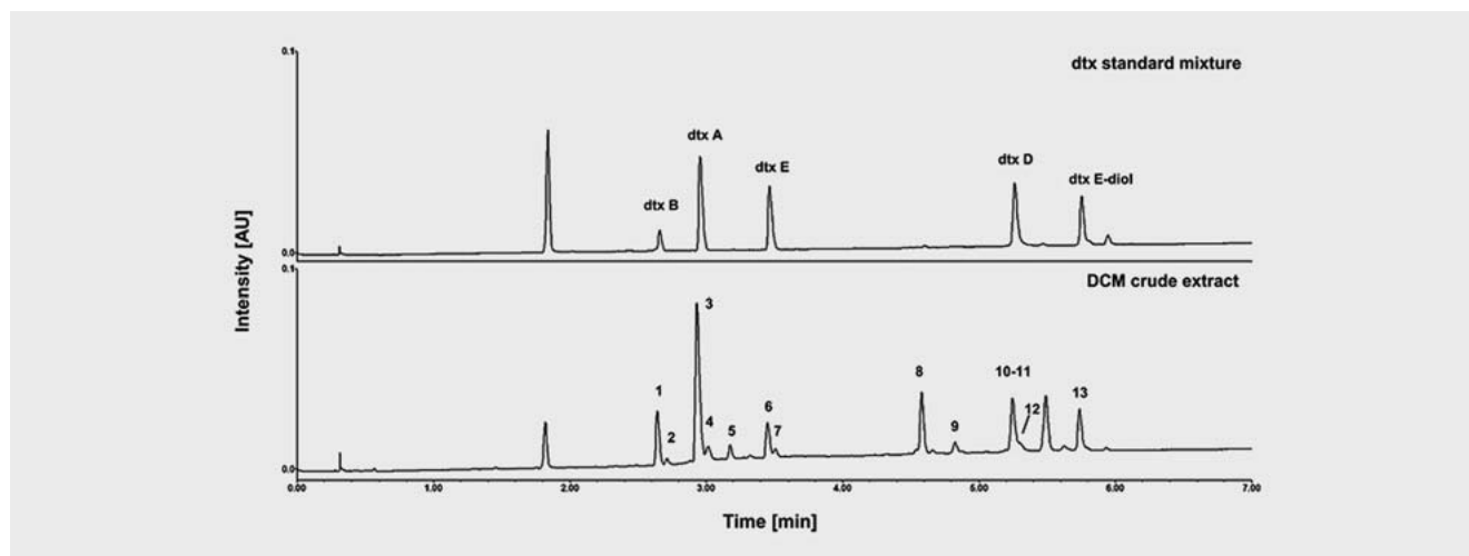
► Fig. 5 Representative UHPSFC-PDA chromatogram of a Metarhizium brunneum DCM crude extract and a destruxine standard mixture containing dtx A, B, D, E, and E-diol. Reproduced with permission from [63].
