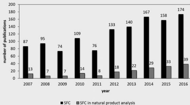
► Fig. 2 Number of publications per year in the field of SFC in general and of SFC in natural product analysis over the last 10 years. Source: Scifinder. Date of information gathering: May 2017.
