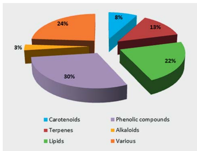
► Fig. 1 Range of SFC applications in natural product analysis categorized by substance classes from 2012 to 2016. Scifinder. Date of information gathering: May 2017.
