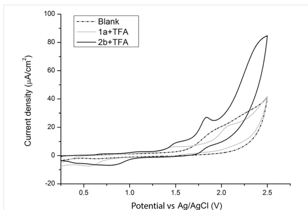
Figure 1 Cyclic voltammograms using n -Bu 4 NBF 4 (0.1 M) as electrolyte in TFE at 20 mV s -1 , under N 2 . Working electrode: glass carbon; reference electrode: Ag/AgCl in 3 M NaCl; auxiliary electrode: Pt wire. Blank (dots); 1a with 3 eq of TFA (gray); 2b with 3 eq of TFA (black).
