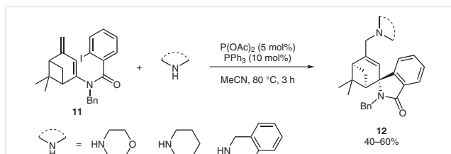
Scheme 9 Racemic intramolecular arylation/amination
