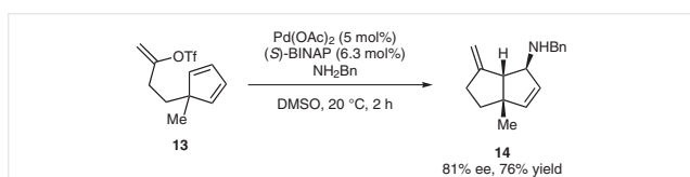
Scheme 10 Enantioselective intramolecular vinylation/amination
