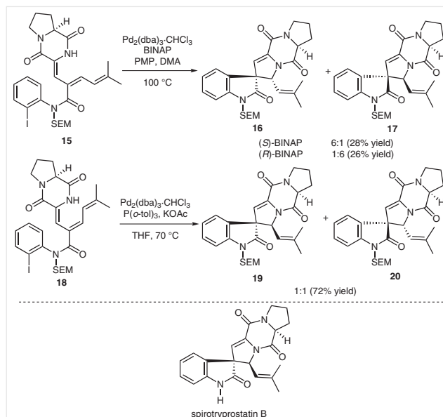
Scheme 11 Enantioselective intramolecular arylation for the total synthesis (–)-spirotryprostatin B
