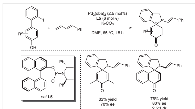
Scheme 38 Preliminary studies on asymmetric reaction
