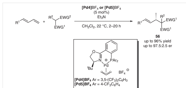
Scheme 39 Enantioselective hydroalkylation
