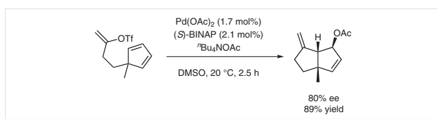
Scheme 44 Enantioselective intramolecular vinyloxygenation
