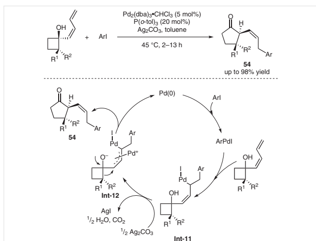
Scheme 36 Cascade insertion–ring expansion reaction of 1,3-dienylcyclobutanols with aryl iodides for the synthesis of ( Z )-2-(3-aryl-1-propenyl)cyclopentanones
