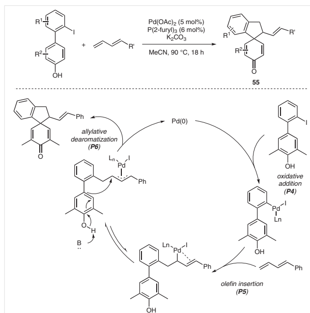
Scheme 37 Dearomatization reaction of phenol-derived biaryls with 1,3-dienes for the synthesis of spirocyclic compounds
