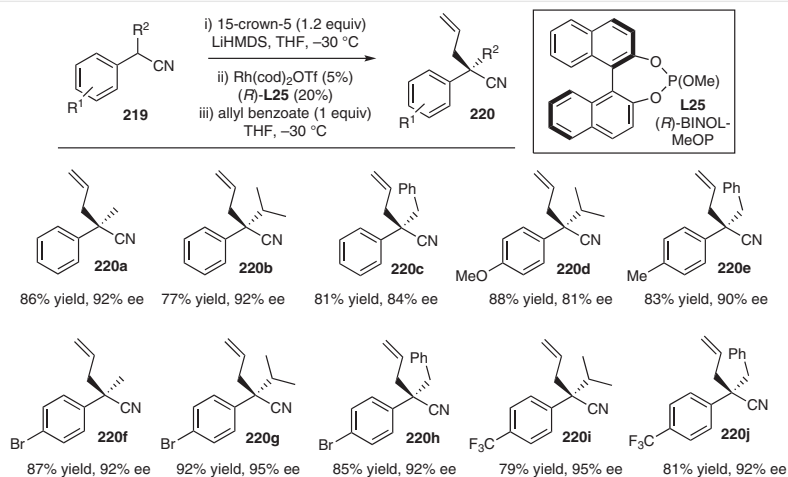
Scheme 76 Rh-catalyzed asymmetric alkylation of secondary benzylic nitriles
