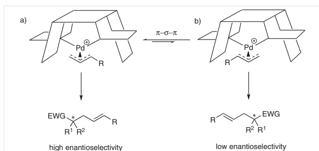
Scheme 61 Rationale for higher enantioselectivity for alkylation of 3-substituted electrophiles
