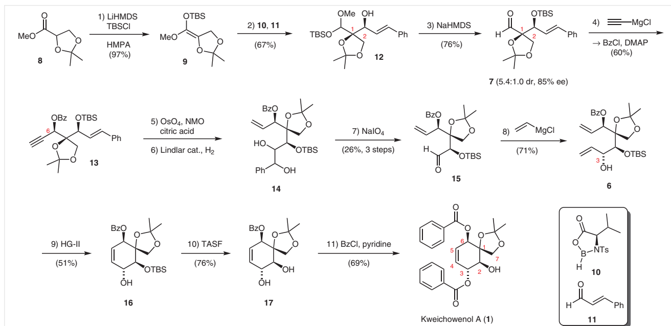
Scheme 2 Asymmetric synthesis of kweichowenol A. Reagents and conditions: 1) TBSCl, LiHMDS, THF/HMPA, -78^{\circ}\text{C} \rightarrow 0^{\circ}\text{C} , then 8 , -78^{\circ}\text{C} ; 2) N -Ts- D -valine, \text{BH}_3\cdot\text{THF} , \text{CH}_2\text{Cl}_2 , 0^{\circ}\text{C} \rightarrow \text{rt} , then 11 , 9 , -78^{\circ}\text{C} ; 3) NaHMDS, THF, -78^{\circ}\text{C} \rightarrow 0^{\circ}\text{C} ; 4) ethynylmagnesium chloride, THF, -78^{\circ}\text{C} \rightarrow 0^{\circ}\text{C} , then BzCl, DMAP, 0^{\circ}\text{C} \rightarrow \text{rt} ; 5) \text{OsO}_4 , NMO, citric acid, t -BuOH/acetone/ \text{H}_2\text{O} , 60^{\circ}\text{C} ; 6) Lindlar cat., \text{H}_2 , EtOAc/pyridine; 7) \text{NaIO}_4 , THF/ \text{H}_2\text{O} ; 8) vinylmagnesium chloride, THF, -78^{\circ}\text{C} \rightarrow 0^{\circ}\text{C} ; 9) HG-II, PhMe, 50^{\circ}\text{C} ; 10) TASF, DMF; 11) BzCl, pyridine, -27^{\circ}\text{C} \rightarrow -20^{\circ}\text{C} . DMAP = 4-(dimethylamino)pyridine, HG-II = second-generation Hoveyda–Grubbs catalyst, HMDS = bis(trimethylsilyl)amide, HMPA = hexamethylphosphoramide, NMO = N -methylmorpholine N -oxide, TASF = tris(dimethylamino)sulfonium difluorotrimethylsilicate, TBS = tert -butyldimethylsilyl.
