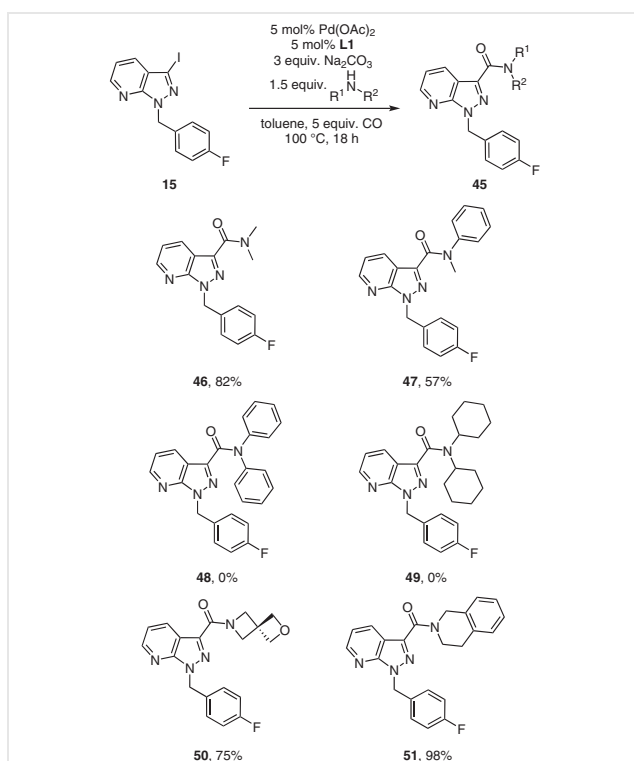
Scheme 3 Extension of general aminocarbonylation protocol to the synthesis of N-1-substituted pyrazolo[3,4- b ]pyridine tertiary amide derivatives 46–51 . Reagents and conditions: aryl iodide 15 (0.28 mmol), amine (0.42 mmol), Pd(OAc) 2 (5 mol%), Xantphos (5 mol%), Na 2 CO 3 (3 equiv.), toluene (0.56 mL), CO surrogate (5 equiv.), 100 °C, 18 h.
