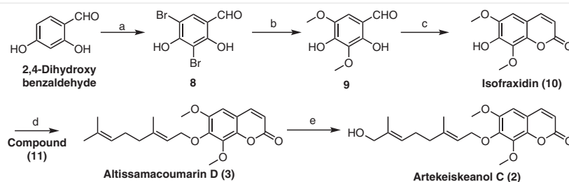
Scheme 3 Reagents and conditions: (a) Br 2 , EtOH, r.t., 1 h, 98%; (b) NaOMe, CuCl, DMF, reflux 8 h, 75%; (c) C2-Ylide, N,N -diethylaniline, reflux, 12 h, 72%; (d) Geranyl bromide ( 11 ), K 2 CO 3 , KI (cat), DMF, r.t., 2 h, 80%; (e) SeO 2 , TBHP/CH 2 Cl 2 (2:1), 0 °C to r.t., 4 h, 63%.
