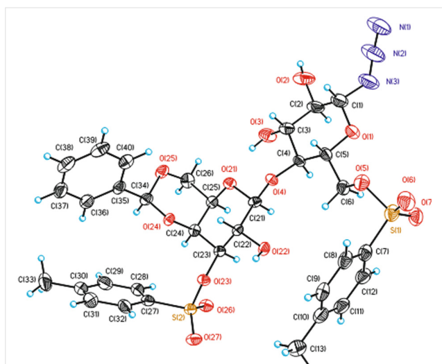
Figure 1 X-ray crystal structure of bistosylate 17
