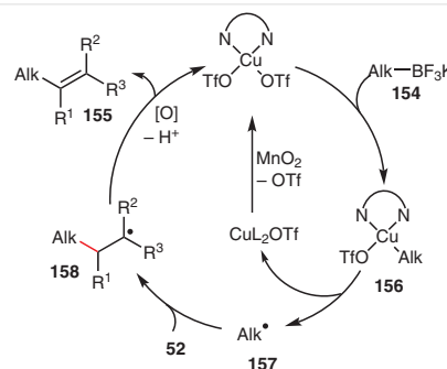
Scheme 27 Chemler's mechanism for the Cu-catalyzed Heck reaction of alkyl trifluoroborates
