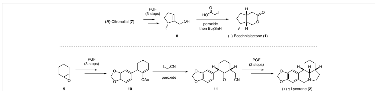
Scheme 2 Strategy for the synthesis of 1 and 2
