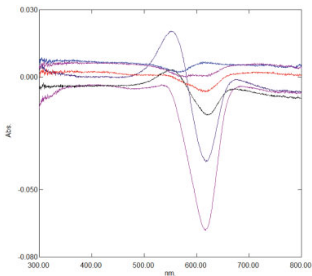
Fig. 3 Difference spectrum of 50 \mu M MV in 20 mM citrate buffer pH 4.0 with control added to the reference cuvette and Glycerol 50 M added to the sample cuvette. Spectra correspond to t = 0 , t = 10 minutes, t = 100 minutes, t = 260 minutes, t = 4 days and t = 11 days after mixing (see text for details). MV, methylene violet (Berntsen).
