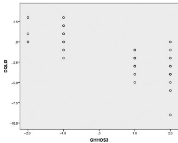
Fig. 4 Scatter plot showing correlations between GHHOS and DLQI change over 3 months for VM sample ( n = 74 ); r = -0.776 (strong negative linear relationship); p < 0.001^* .
