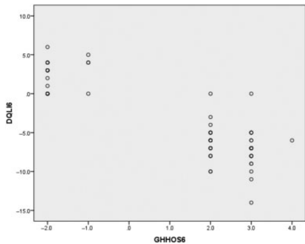
Fig. 5 Scatter plot showing correlations between GHHOS and DLQI change over 6 months for VM sample ( n = 74 ); r = -0.875 (strong negative linear relationship); p < 0.001^* .
