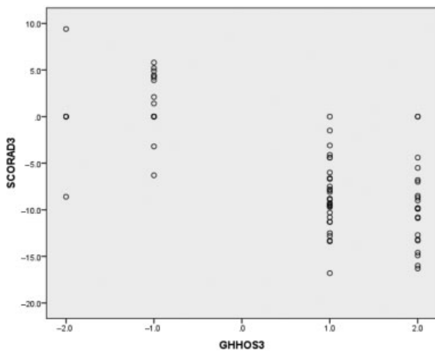
Fig. 2 Scatter plot showing correlations between GHHOS and SCORAD change over 3 months for VM sample ( n = 74 ); r = -0.723 (strong negative linear relationship); p < 0.001^* .
