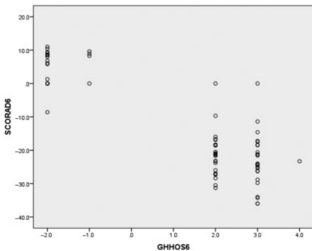
Fig. 3 Scatter plot showing correlations between GHHOS and SCORAD change over 6 months for VM sample ( n = 74 ); r = -0.869 (strong negative linear relationship); p < 0.001^* .
