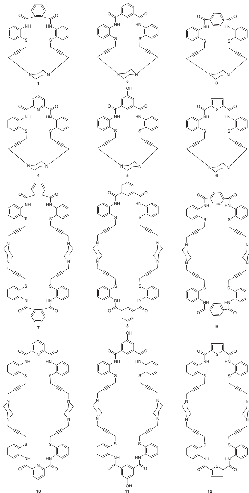
Figure 1 Structures of piperazinoamide based 1:1 and 2:2 oligomeric forms of macrocycles 1–12
