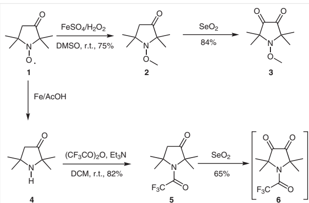
Scheme 2 Synthesis of precursors of 1-oxyl-2,2,5,5-tetramethylpyrrolidine-3,4-dione
