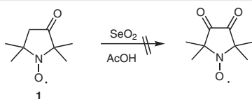
Scheme 1 Attempted synthesis of a paramagnetic diketone
