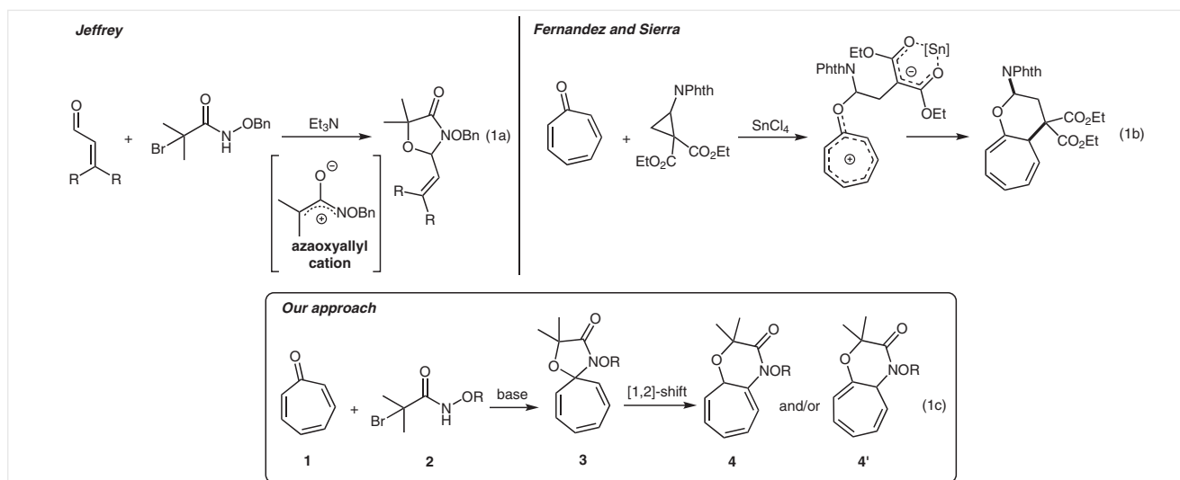
Scheme 1 [8+3] Annulation between tropone and azaoxyallyl cation
