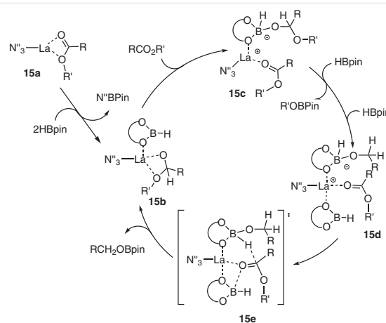
Scheme 15 Proposed mechanism for ester hydroboration
