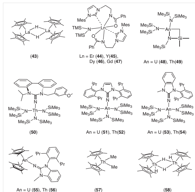
Figure 5 Organolanthanide and organoactinide complexes for imine and nitrile hydroborations
