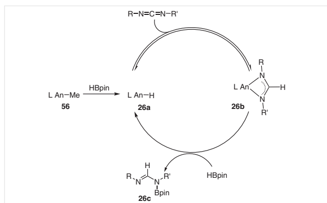
Scheme 26 Proposed mechanism for hydroboration of carbodiimides
