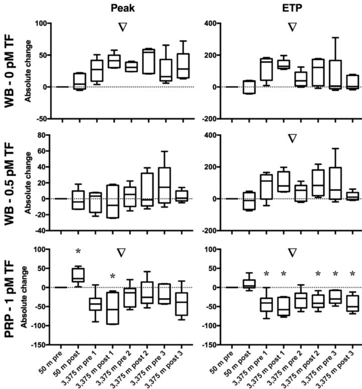
Fig. 3 Influence of normoxic and hypoxic exercises on thrombin generation (TG) in whole blood (WB) and platelet-rich plasma (PRP). TG was measured before and after 2 hours of strenuous exercise, once at 50 m altitude and three times at 3,375 m altitude, in whole blood (WB) and PRP. Parameters derived from the TG curve are peak height (peak in nM or % of NPP) and endogenous thrombin potential (ETP in nM-min or % of NPP). N = 6 , one measurement is missing (subject 5, WB TG post 3). Results are expressed as the absolute change of 50 m pre-exercise; a value above 0 indicates an increase, and a value below 0 indicates a decrease. \nabla = p < 0.05 (Friedman's test); * = p < 0.05 compared with zero (Wilcoxon signed-rank test).
