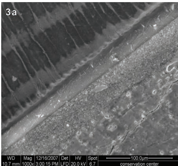
Figure 3. a. SEM micrograph of thermocycled Calibra Resin Cement and b. its corresponding EDAX spectrum curve at one point along the tooth/restoration interface.
