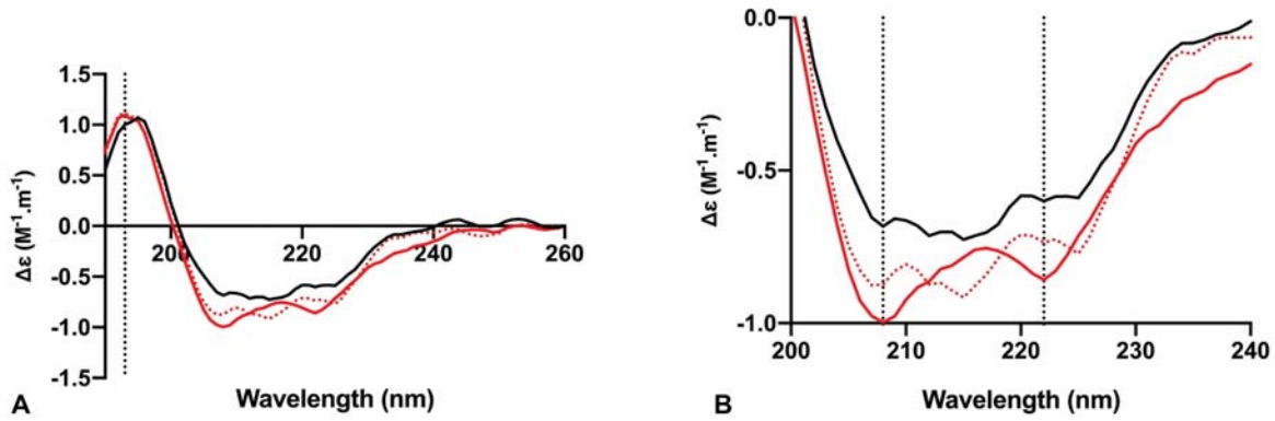
Fig. 4 The conformational change of the SARS-CoV-2 S1 RBD observed in the presence of heparin by CD spectroscopy. (A) Circular dichroism spectra (190–260 nm) of SARS-CoV-2 S1 RBD alone (black solid line) and with heparin (red solid line) in PBS, pH 7.4. The red, dotted line represents the sum of the two individual spectra and the fact that this is distinct from the spectrum of the RBD with heparin (red solid line) indicates that a conformational change and, therefore, binding have occurred. The dotted vertical line indicates 193 nm. (B) Details of the same spectra expanded between 200 and 240 nm. Vertical dotted lines indicate 222 and 208 nm. PBS, phosphate buffered saline; RBD, receptor-binding domain.
