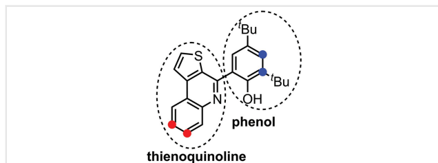
Figure 1 Chromophore 1 with its thienoquinoline as well as phenol substructure highlighted and the sites of ring fusion to the bicyclo [2.2.2]octane scaffold in red (at the thienoquinoline part) and blue (at the phenolic part).
