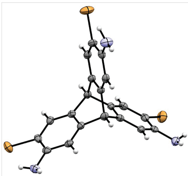
Figure 2 Single crystal X-ray structure of triptycene 4 as ORTEP plot with thermal ellipsoids at the 50% probability level. Carbon: grey; hydrogen: white; nitrogen: blue; bromine: light brown.
