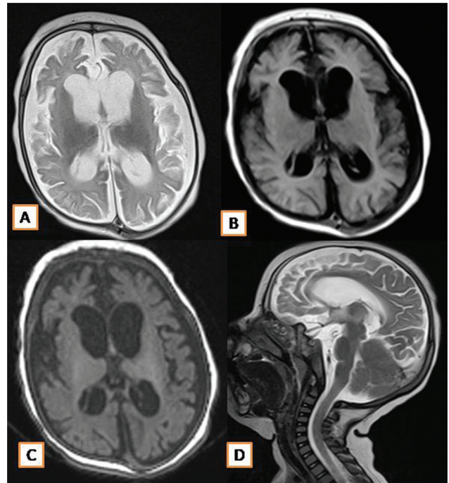
Fig. 6 Magnetic resonance imaging brain axial T2-weighted imaging, T1-weighted imaging, fluid-attenuated inversion recovery, and sagittal T2-weighted imaging showing a loss of deep white matter volume evidenced by thinning of gyri and prominent sulcal spaces in bilateral cerebral hemispheres resulting in diffuse cerebral atrophy. Resultant dilatation of the ventricular system noted. There is severe thinning of corpus callosum.
