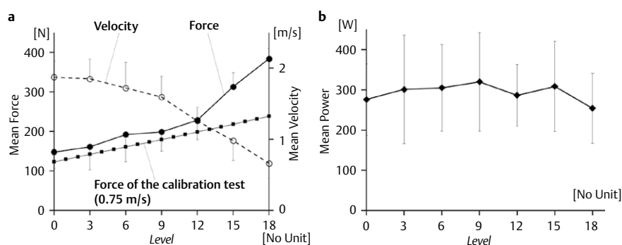
► Fig. 5 Averaged forces ( a ), velocities ( a ), and powers ( b ) as functions of Level for 14 subjects. These plots are the mean values between two and five seconds after onset of exercises. In a , the results of force in the calibration test (0.75 m/s) were also plotted for comparison between the calibration and the human tests.
