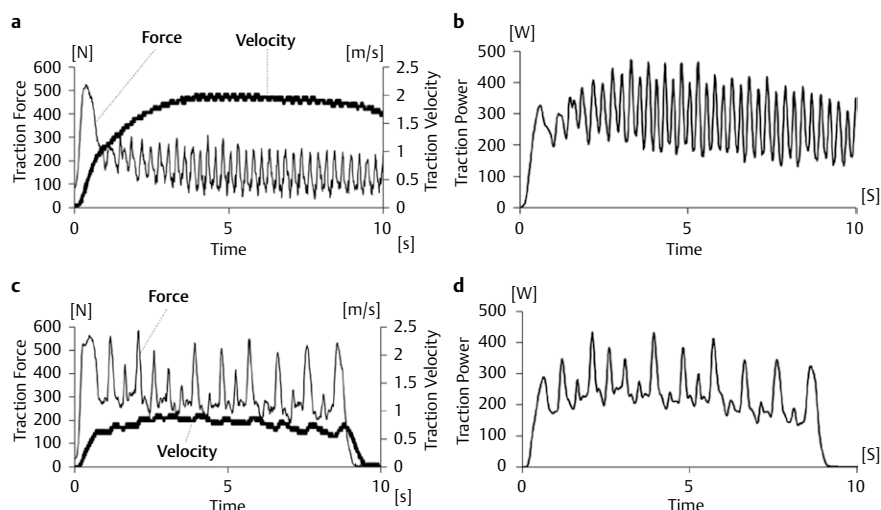
► Fig. 4 Typical examples of time series trajectories of force, velocity ( a and c ), and power ( b and d ), when Level was set relatively low (Level 3, a and b ) and high (Level 15, c and d ), respectively. These data are chosen from a single subject.
