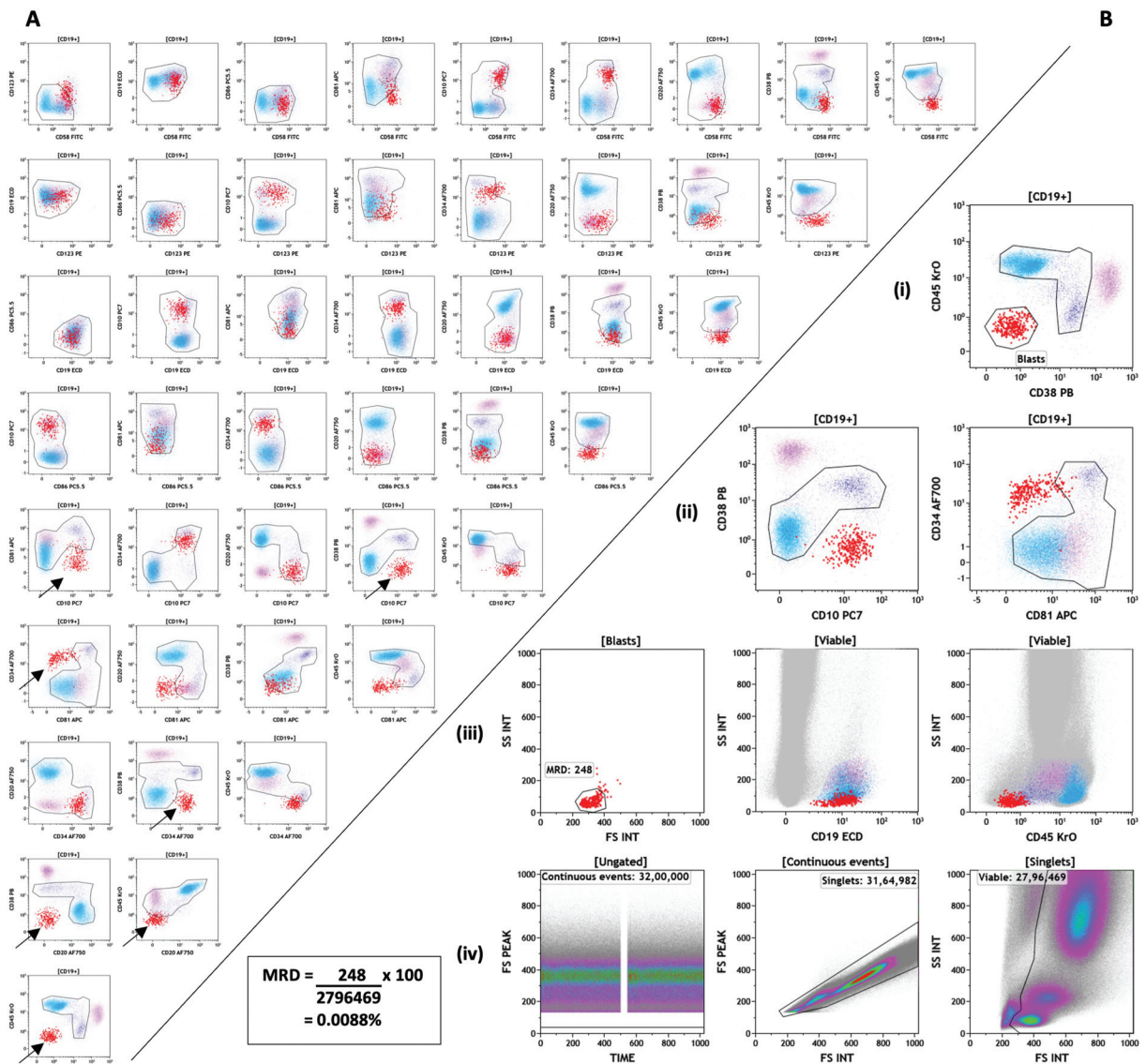
Fig. 2 (A) Panel of plots showing assessment of MRD on bone marrow aspirate sample from a patient of B-ALL at end of induction time point. The mature B cells are shown in light blue color, hematogones in dark blue, and plasma cells are in pink color. The events representing MRD are colored red and depicted in bolder dots than rest of the events. The MRD events are distinctly separate and lying outside the “hematogone-maturation pattern” in some of the plots (indicated by arrows), mostly in lower part of the panel. (B) Representative plots to show calculation of percentage of residual leukemic cells; (i) the residual blasts are gated on CD38 versus CD45 plot (red dots) where these show distinctly different expression for the two markers when compared with normal B cells; that is, CD10 versus CD38 and CD81 versus CD34, highlighting their deviation from normal maturation pattern; (ii) the gated residual blasts are shown in two other plots, that is, CD10 versus CD38 and CD81 versus CD34, highlighting their deviation from normal maturation pattern; (iii) forward scatter (FS) versus side scatter (SS) plot showing gating of tight cluster of cells to refine residual blast population which provides the numerator for calculating MRD, and a retrospective depiction of this MRD-cluster on CD19 versus SS and CD45 versus SS plots; (iv) the denominator for calculation of MRD is provided by gating viable cells on FS INT versus SS INT plot after gating continuous events on time versus FS PEAK plot and removing cell-aggregates on FS INT versus FS PEAK plot. The “text box” shows calculation of percentage of residual leukemic cells.
