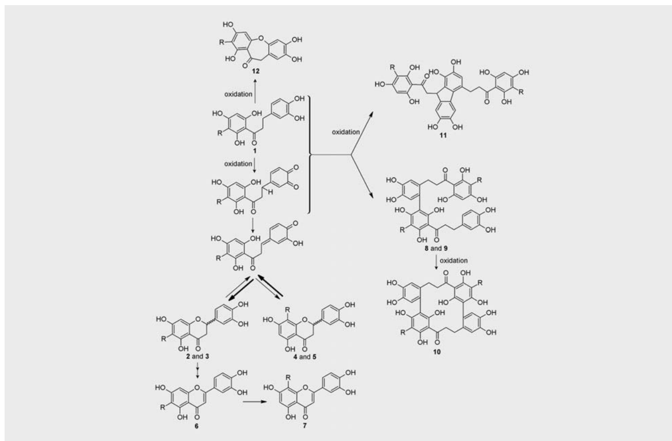
► Fig. 4 Oxidation of aspalathin in the presence of oxygen. [1, aspalathin; 2, ( S )-6-β-D-glucopyranosyleriodictyol; 3, ( R )-6-β-D-glucopyranosyleriodictyol; 4, ( S )-8-β-D-glucopyranosyleriodictyol; 5, ( R )-8-β-D-glucopyranosyleriodictyol; 6, isoorientin; 7, orientin; 8, 9, 10, 11, aspalathin dimers; R = β-D-glucopyranosyl]. Compiled from previous reports [45–47].
