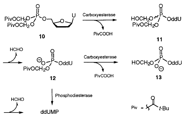
Figure 4. Bis(POM)-nucleotides 10 shown here as their 2',3'-dideoxyuridine derivatives and their degradation pathway
