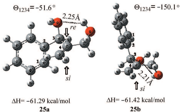
Figure 1 Minimal energy conformations for allylic diol 25
