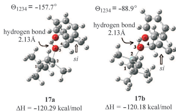
Figure 2 Minimized conformations for the silylated allylic diol 17
